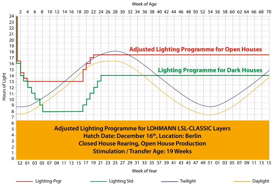
An example of a lighting programme for LOHMANN LSL-CLASSIC Layers adjusted to location, condition and requirements by LOHMANN TIERZUCHT lighting programme tool
