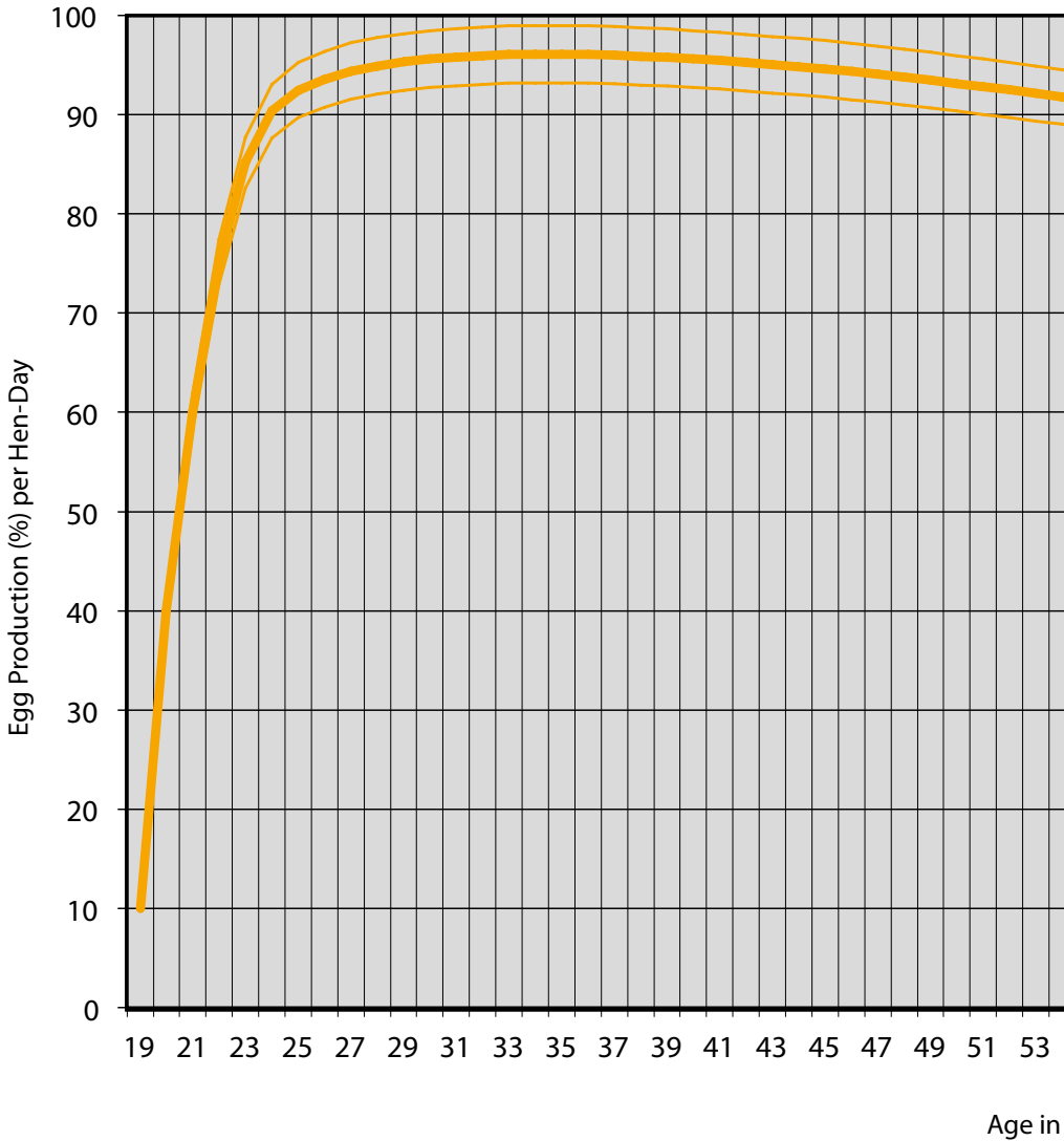
Egg Production Curve for LOHMANN LSL-CLASSIC Layers
